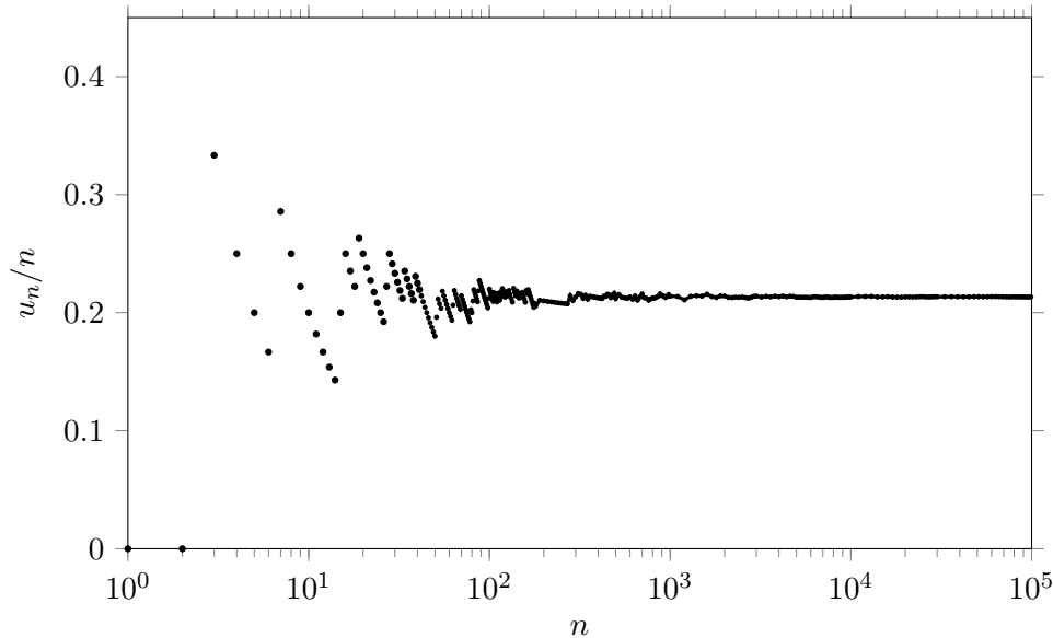
Figure 5.1: The ratio u_n/n against set length n .
